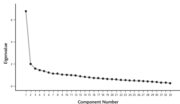
Figure 13: Scree plot
